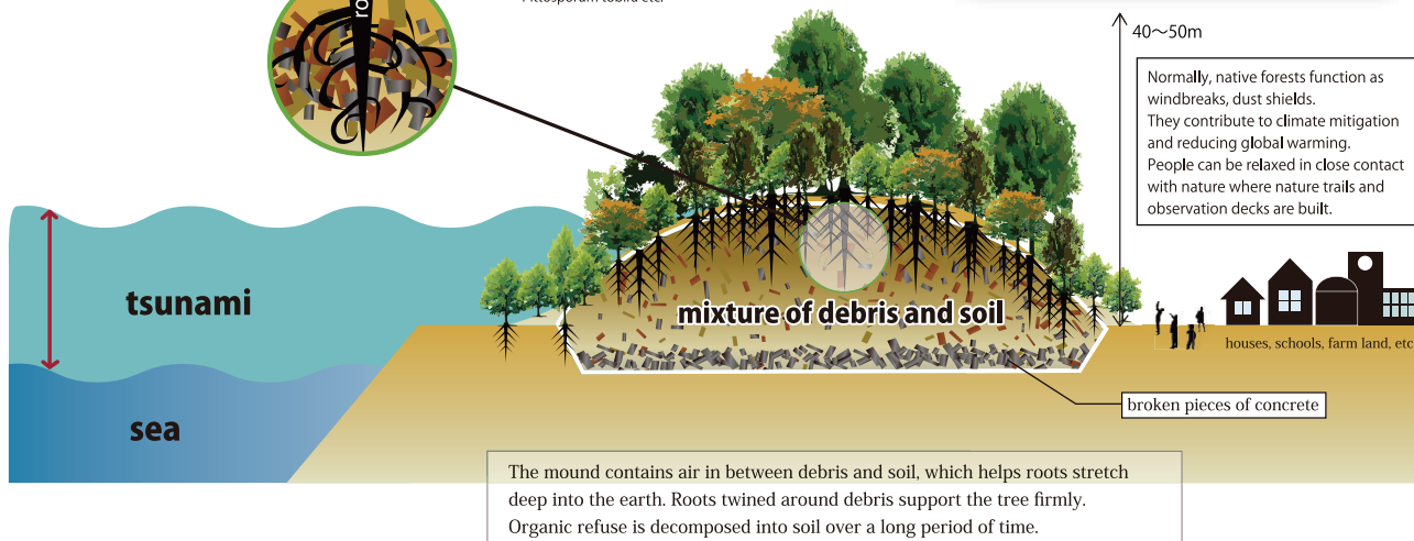
Fig. 2. Proposal of 300 km long tsunami-preventing forest levee (contributed by Rin-no-ji Temple, Sendai).
